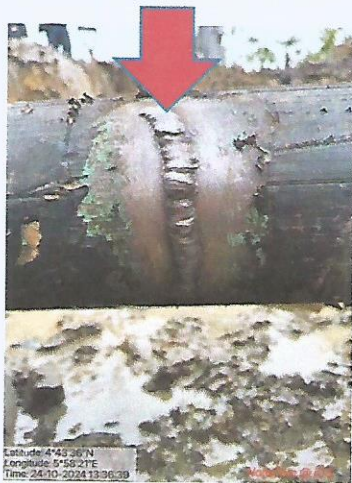
Pic1: Showing one (1no.) 2" valve illegally installed on the pipeline
